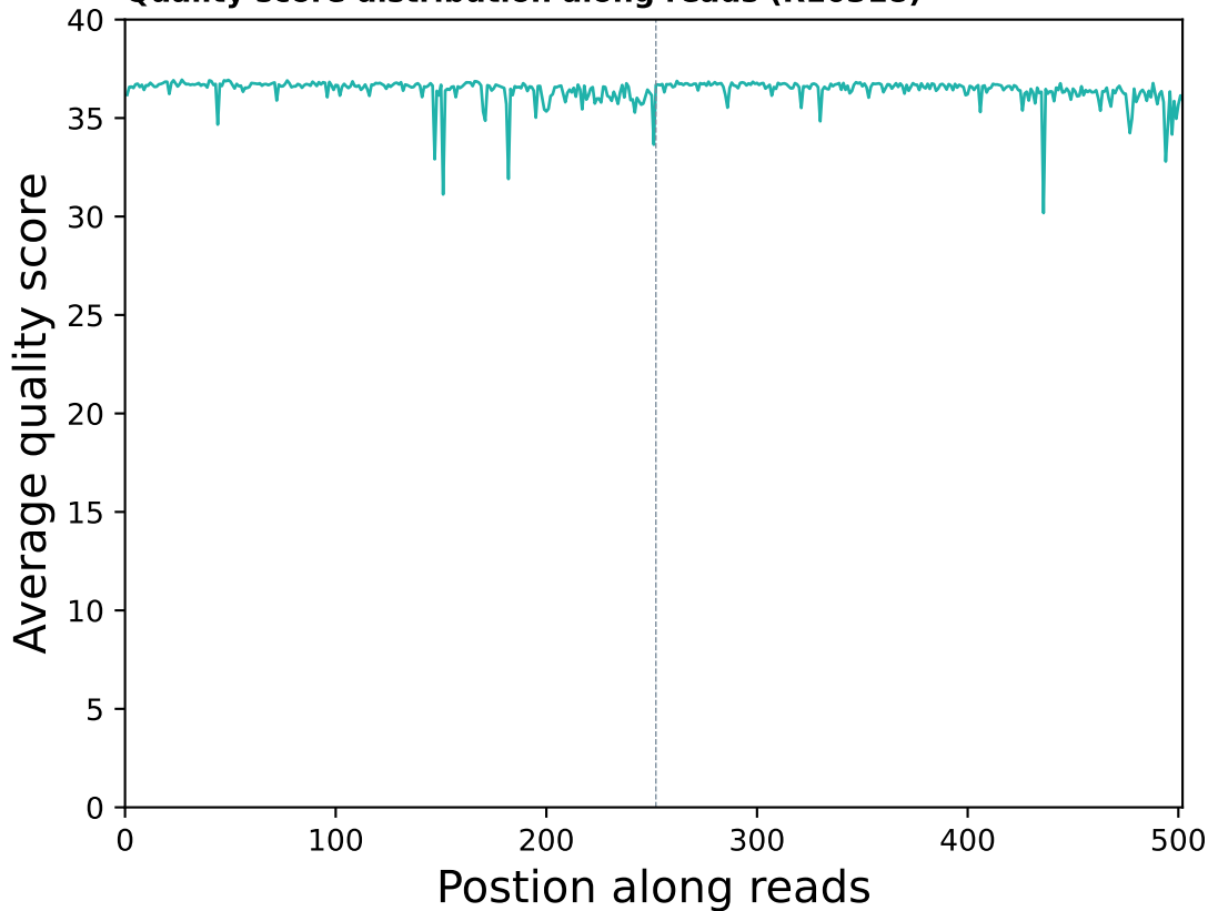
Quality score distribution along reads (R10318)
